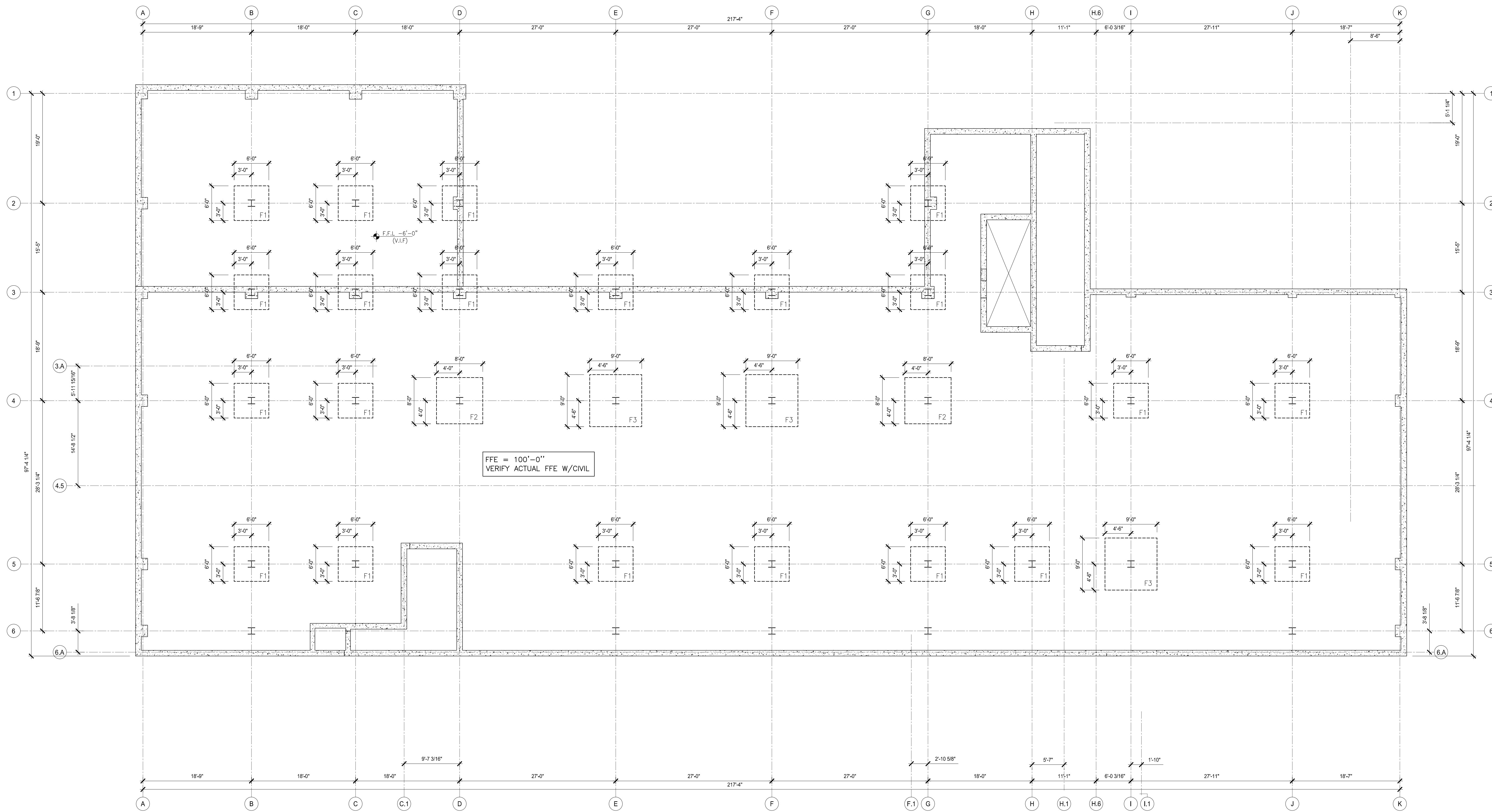
1 BASEMENT FOUNDATION LAYOUT PLAN SCALE: 1/8"=1'-0"
