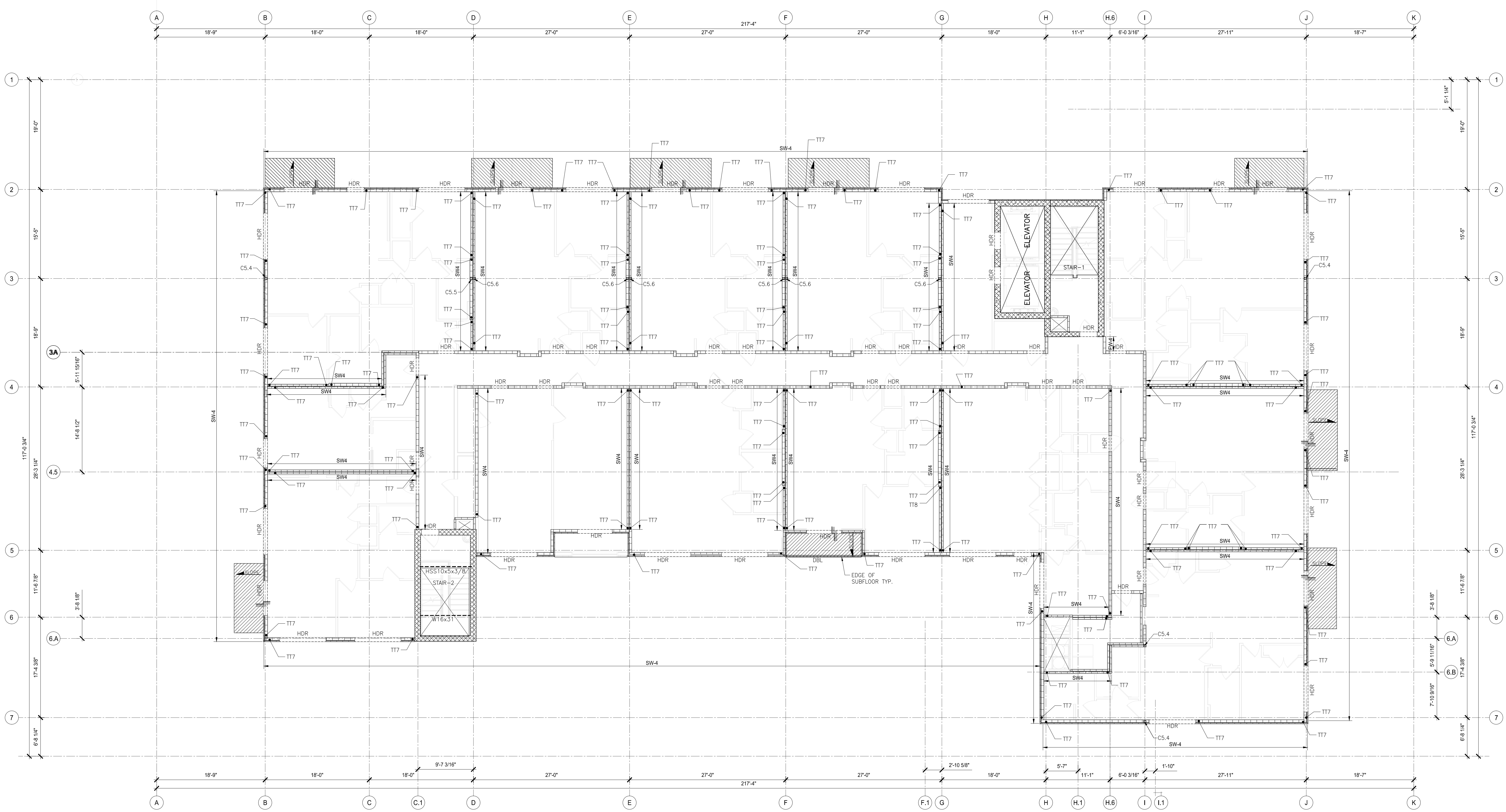
1 5TH FLOOR SHEAR WALL PLAN SCALE: 1/8"=1'-0"
