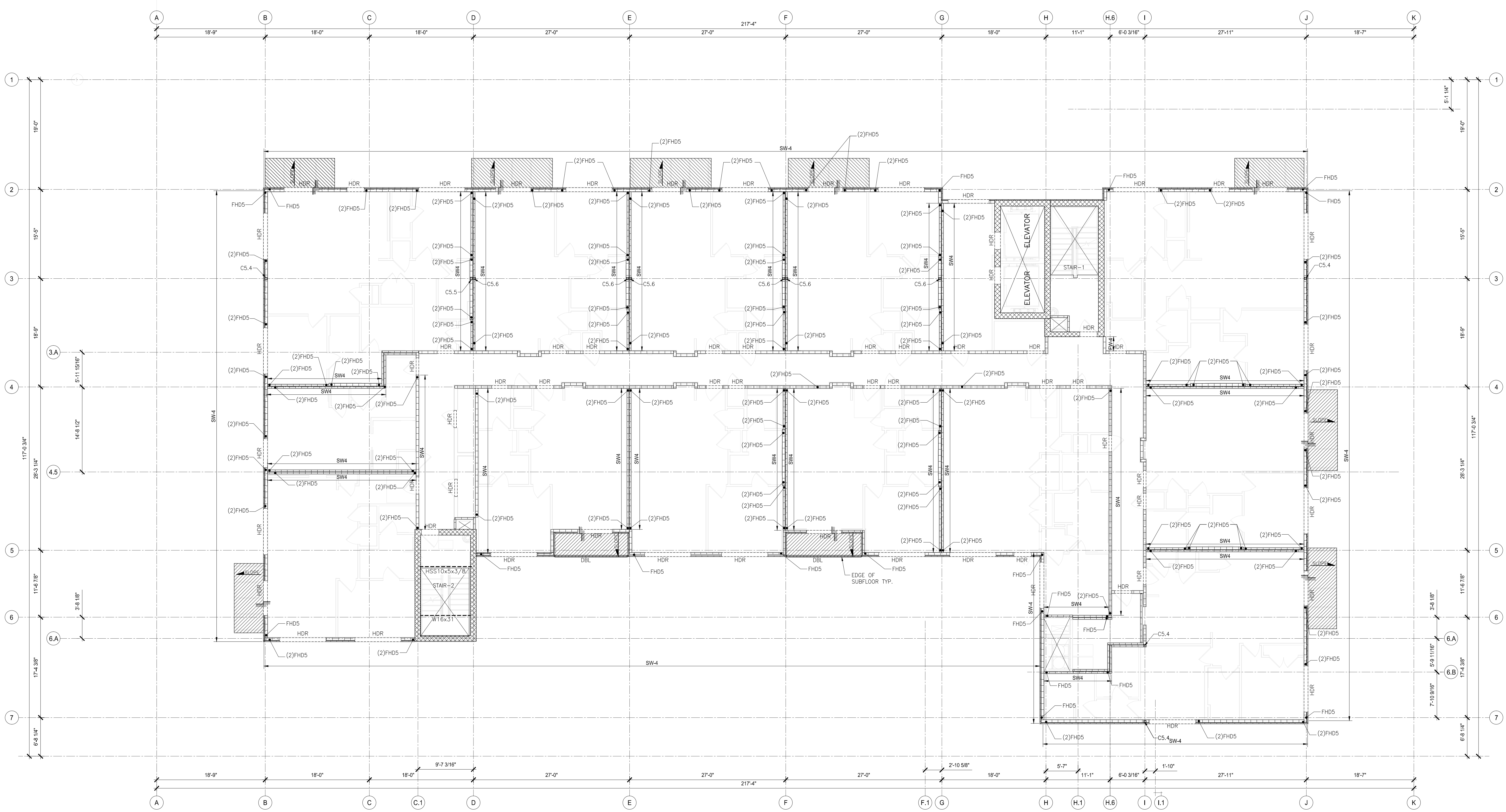
1 3RD FLOOR SHEAR WALL PLAN SCALE: 1/8"=1'-0"
