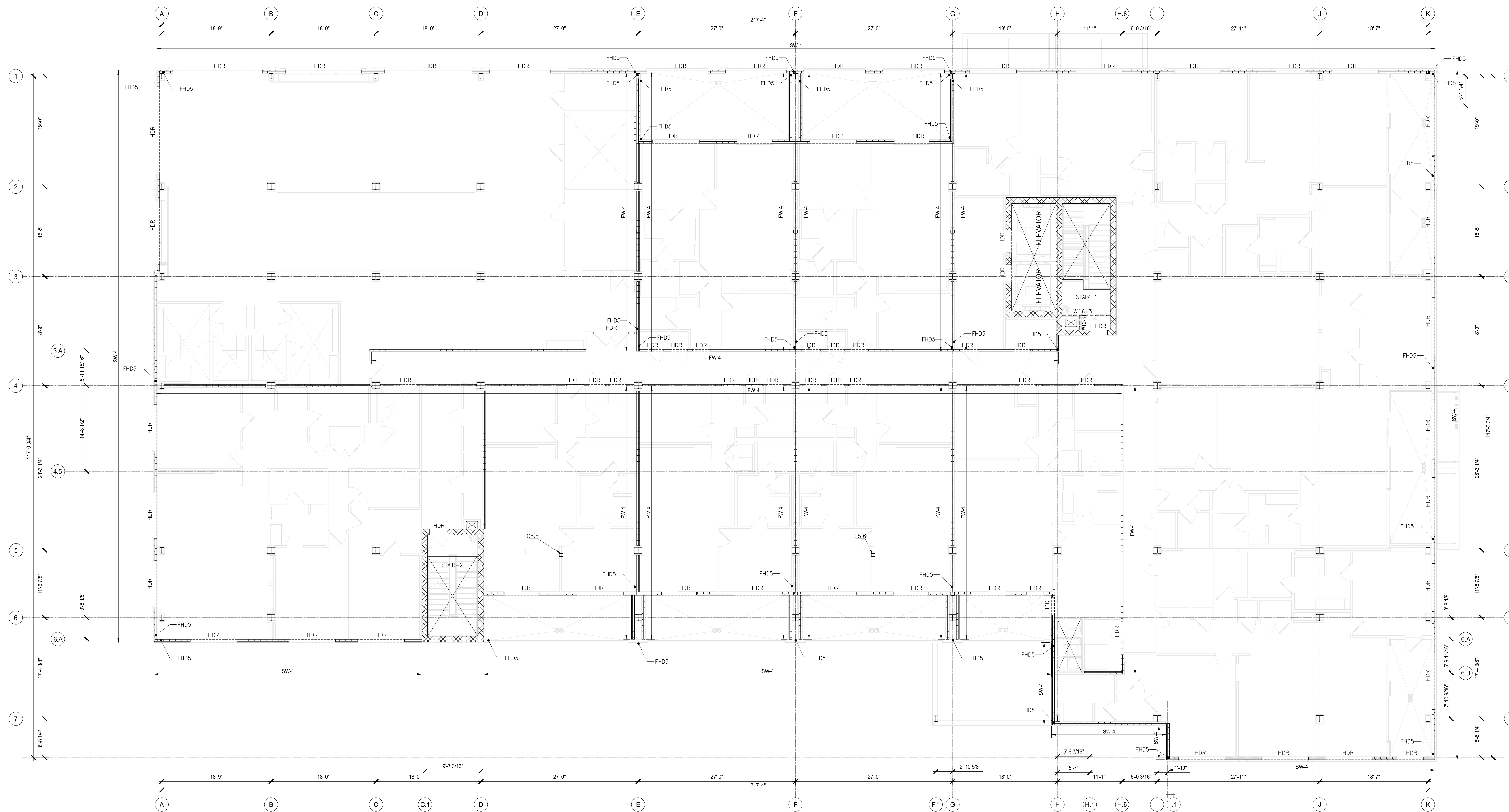
1 2ND FLOOR SHEAR WALL PLAN SCALE: 1/8"=1'-0"
