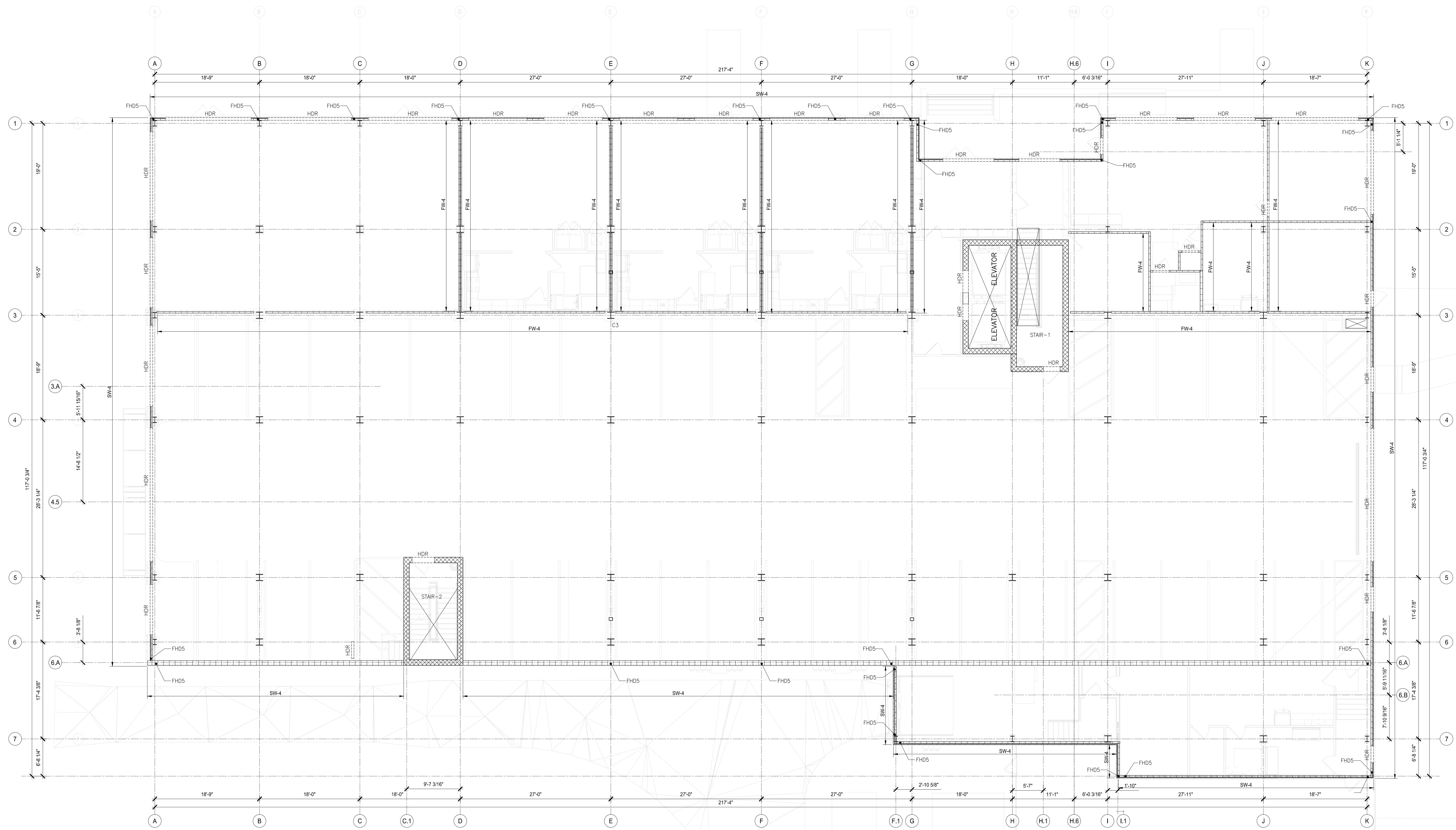
1 1ST FLOOR SHEAR WALL PLAN SCALE: 1/8"=1'-0"
