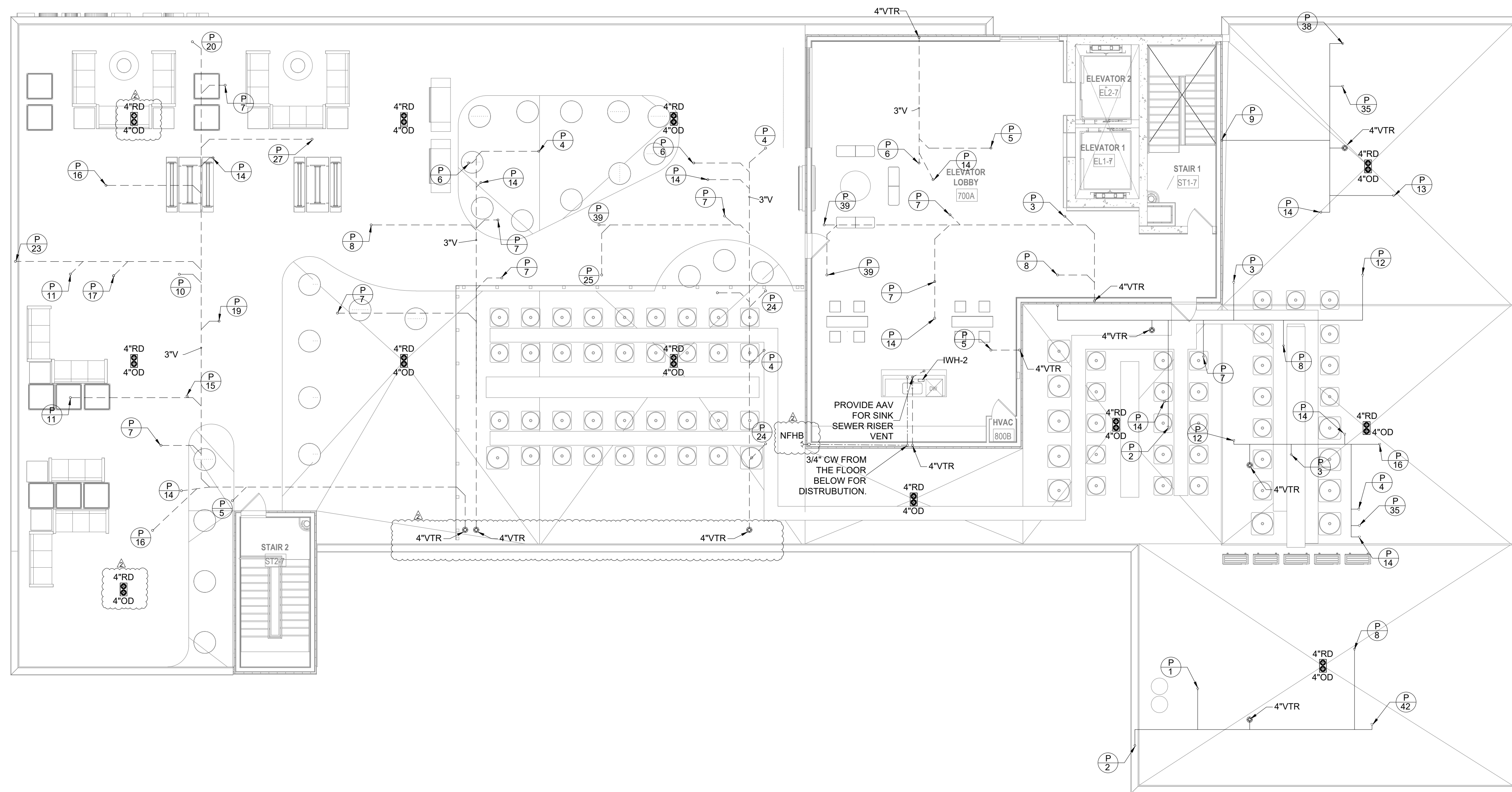
1 BUILDING PLAN - ROOF LEVEL - DRAIN AND VENT LAYOUT 1/8"=1'-0"
