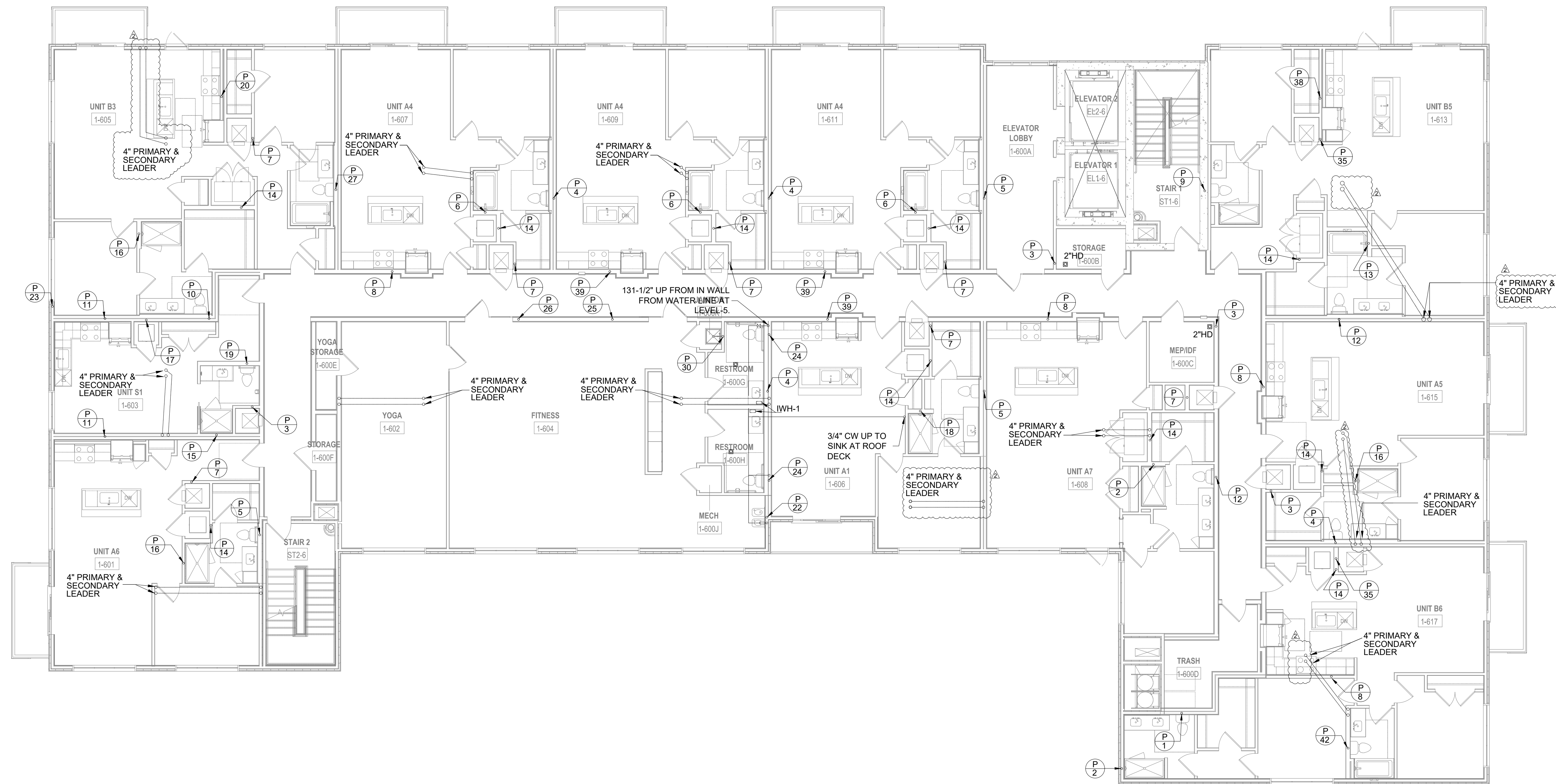
1 BUILDING PLAN - LEVEL 6 - PLUMBING 1/8"=1'-0"
