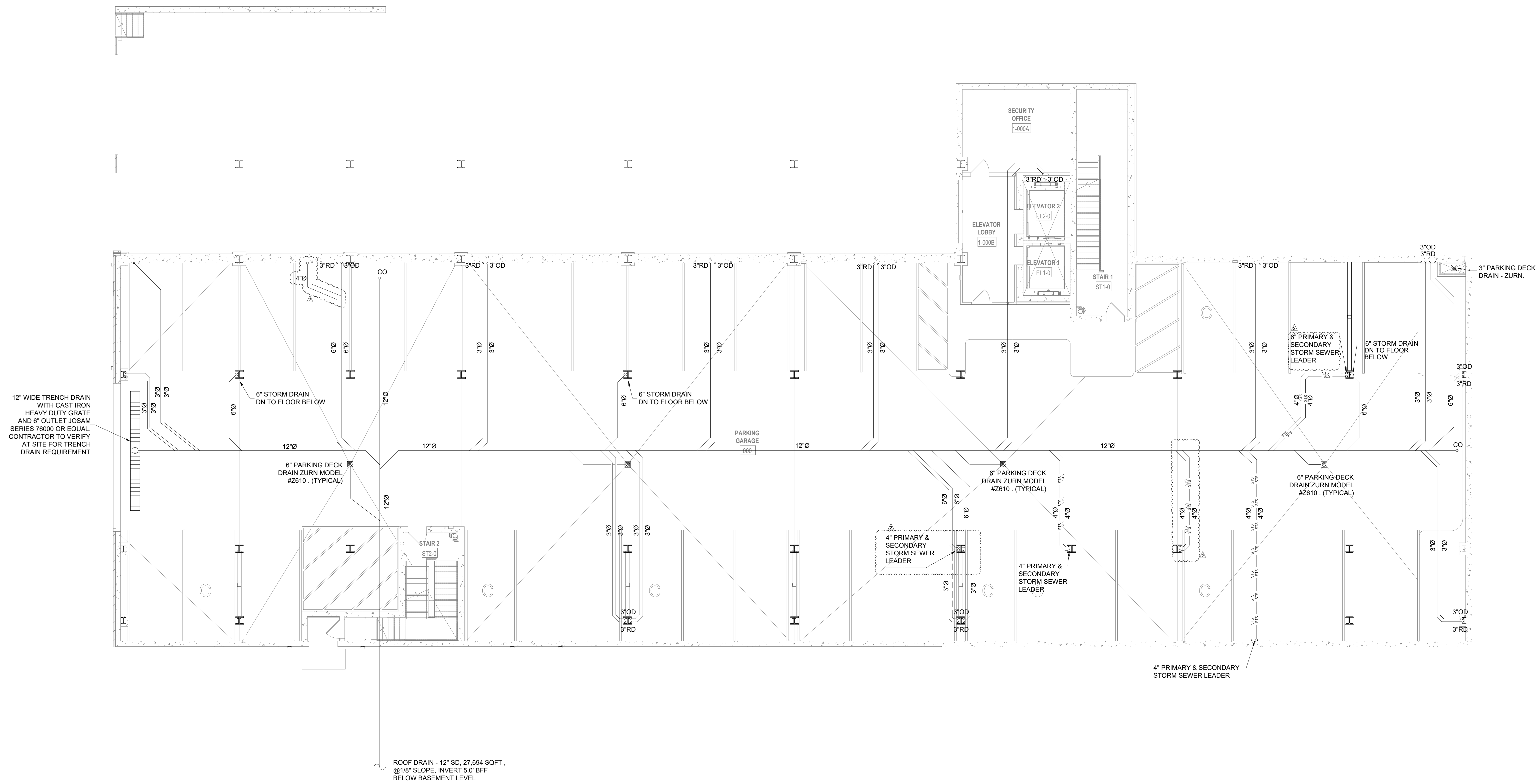
1 BUILDING PLAN - BASEMENT - STORM PLAN 1/8"=1'-0"
