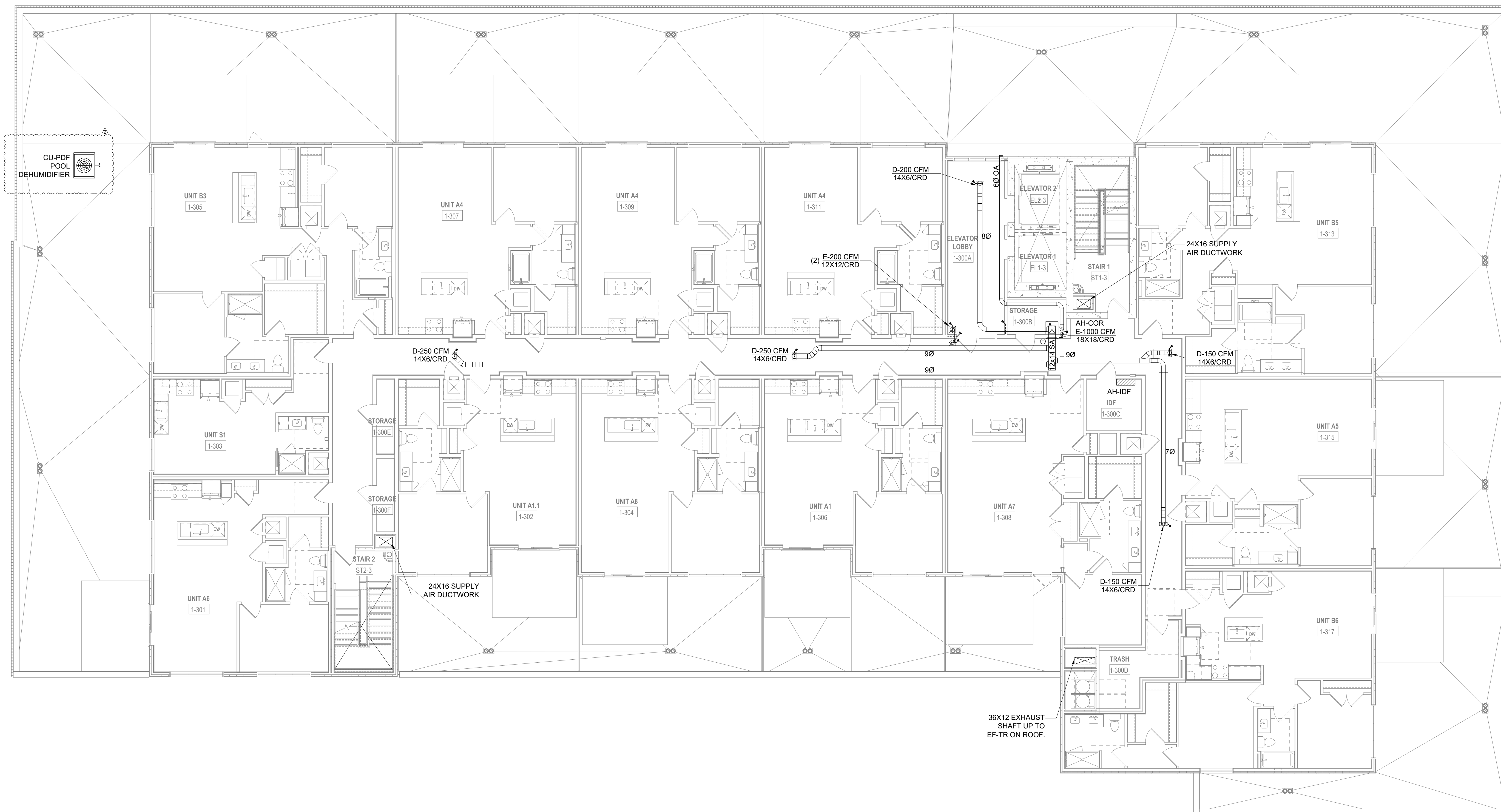
1 BUILDING PLAN - LEVEL 3 - MECHANICAL 1/8"=1'-0"
